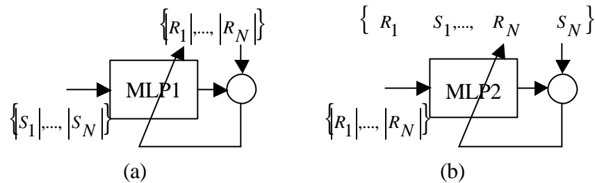
Figure 3. Training of MLPs in the equalizer
