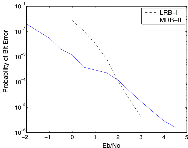
Fig. 7. Performance of LRB-1 and MRB-2 schemes with 6 nodes.
